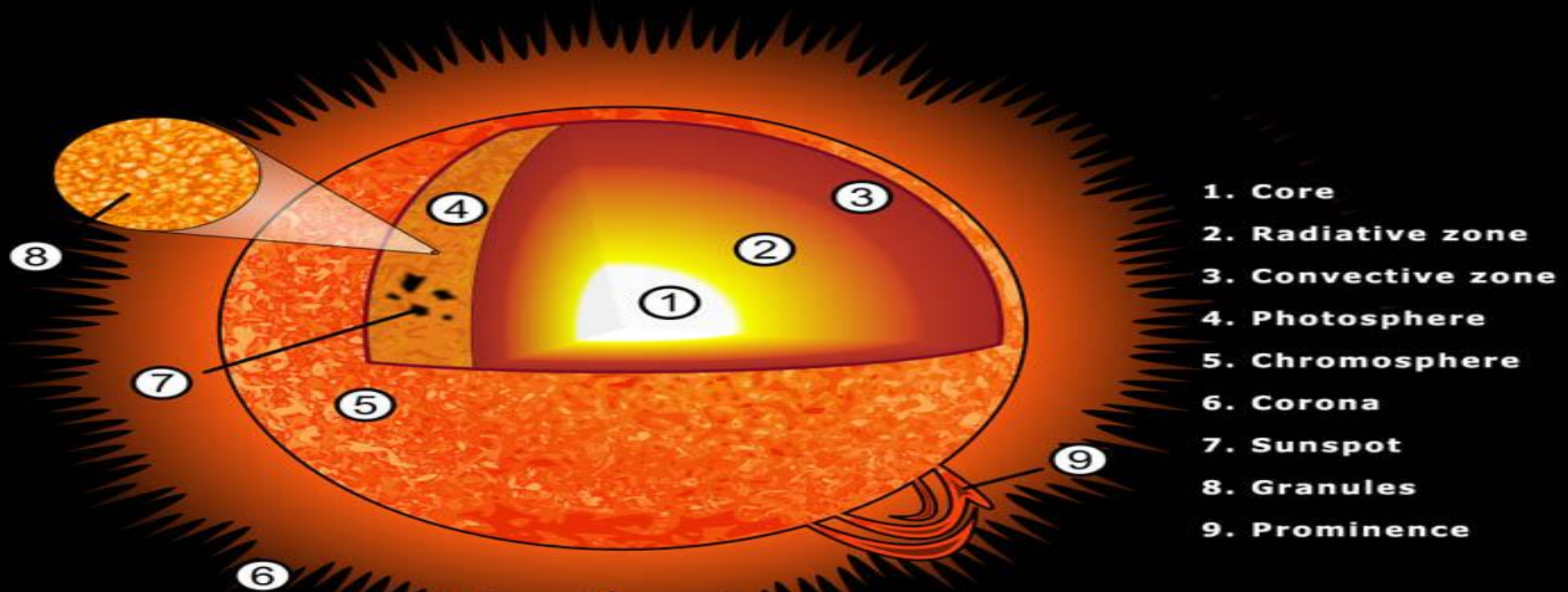
The structure of the Sun
